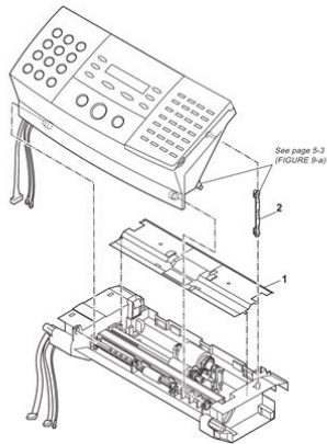
FIGURE 9 READING ASS'Y 2
