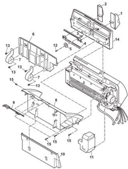
FIGURE 8 READING ASS'Y 1
