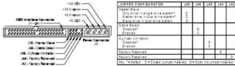
Figure 241 PCB Jumper Location and Configuration
